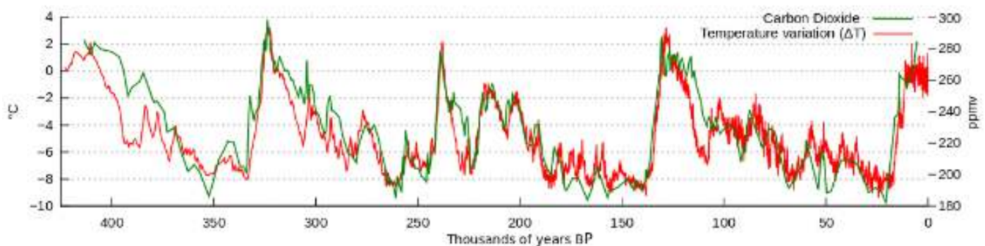
Figure 1 Atmospheric CO 2 and surface air temperature variation over the last ~400,000 years (data from Vostock Ice core, Petit et al., 1999)
