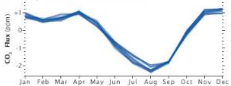
Monthly Change in Carbon Dioxide, 1959-2010
