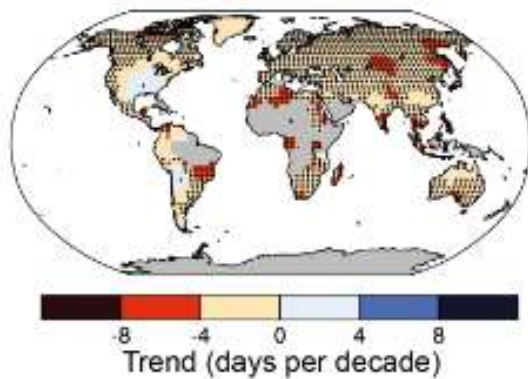
(c) Warm Nights
