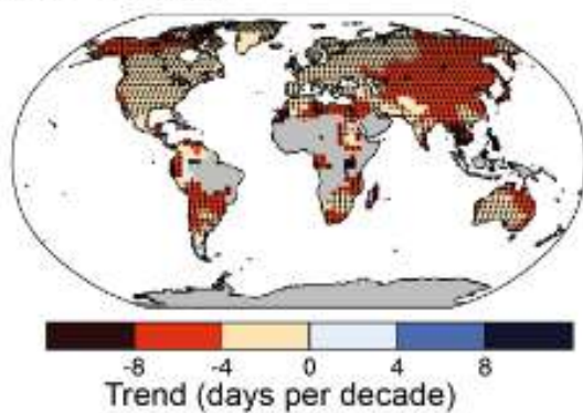
(b) Cold Days
