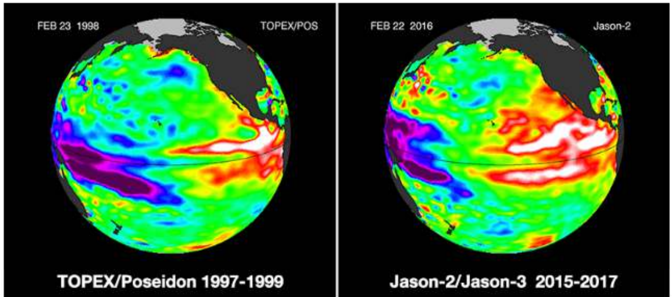
Anomalies of sea surface height (red is positive, blue is negative) in the Pacific ocean during the 1998 and 2016 El Nino events (animation courtesy NASA)
