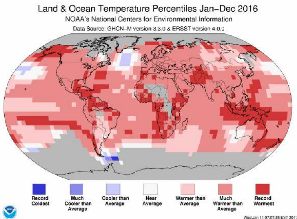
Earth's changing temperatures in 2016 (Image courtesy of NOAA)
