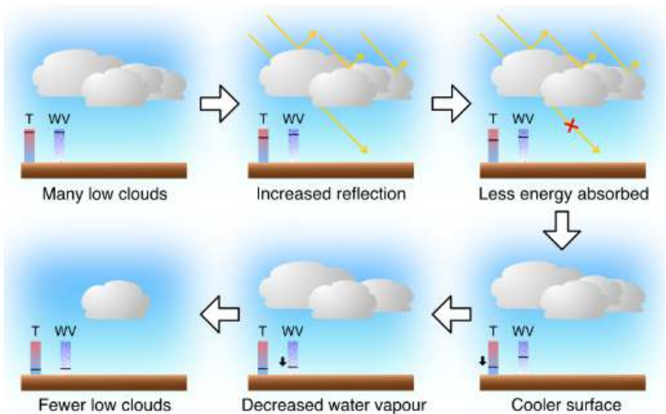
The cloud albedo feedback
