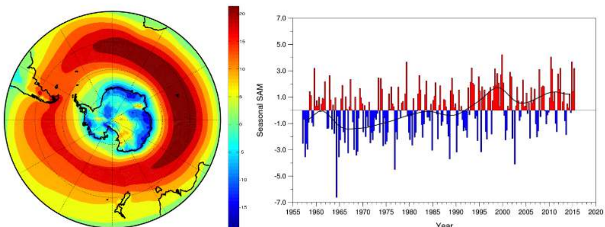
(Left) Annual mean zonal (west-to-east) wind speed in ms-1 (850 hPa) in the Southern hemisphere. (Right) Seasonal SAM index - the black line represents a decadal average (Image courtesy of G. Marshall)
