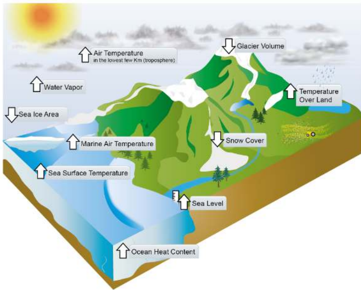
The indicators of a warming world (IPCC, AR5 WG1)
